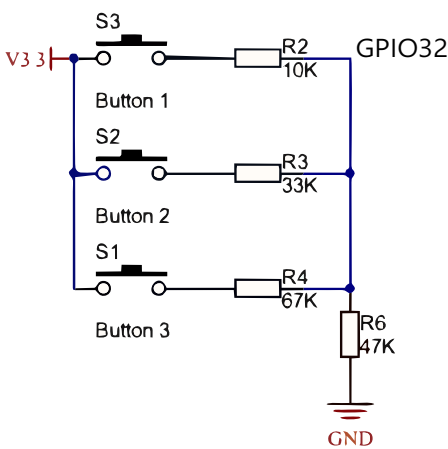
Voltage levels
